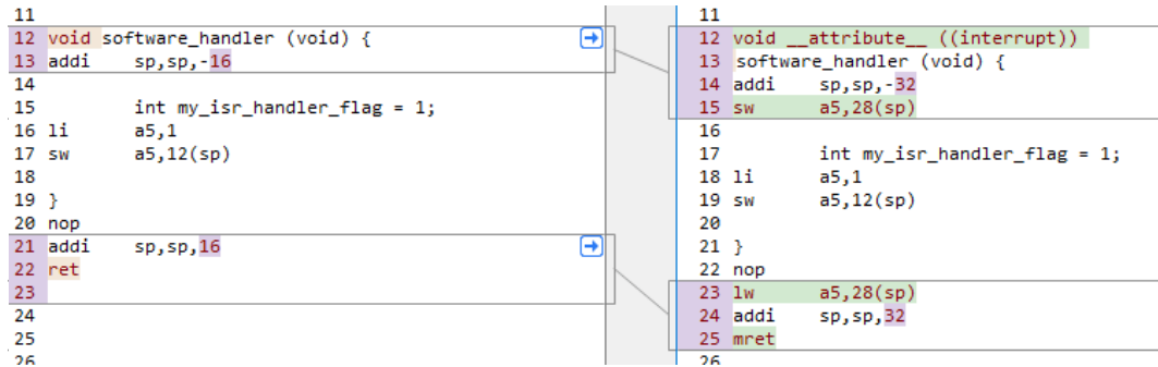
Figure 85: CLINT Interrupt Attribute Example
