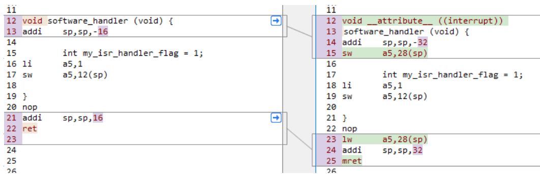
Figure 76: CLIC Interrupt Attribute Example
