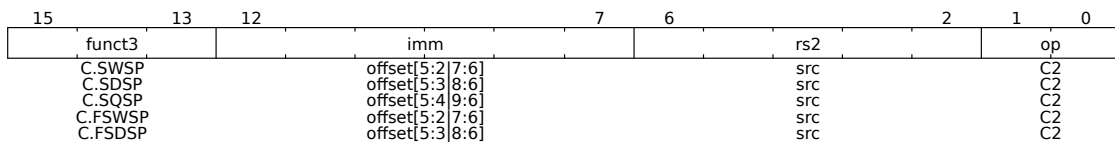
Figure 49: Stack-Pointed-Based Stores
