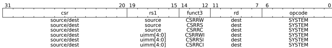
Figure 64: Zicsr Instructions
