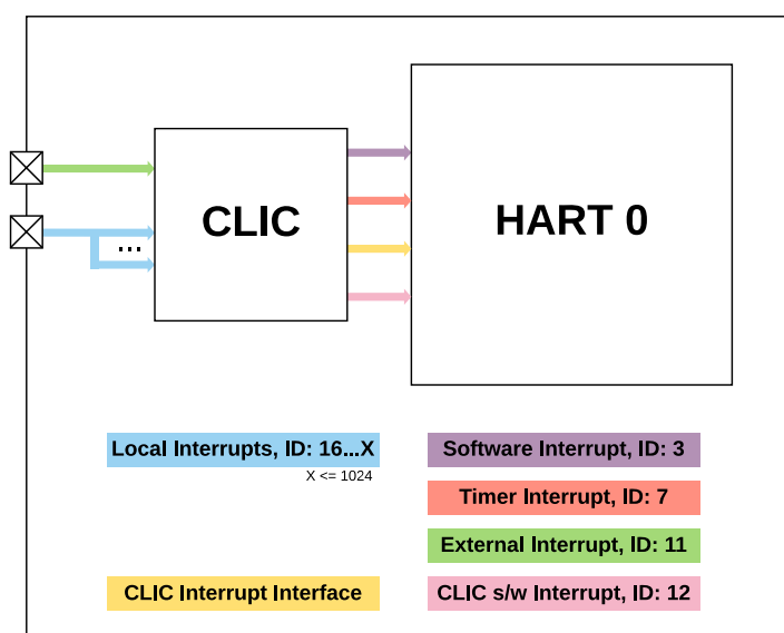
Figure 74: CLIC Block Diagram
