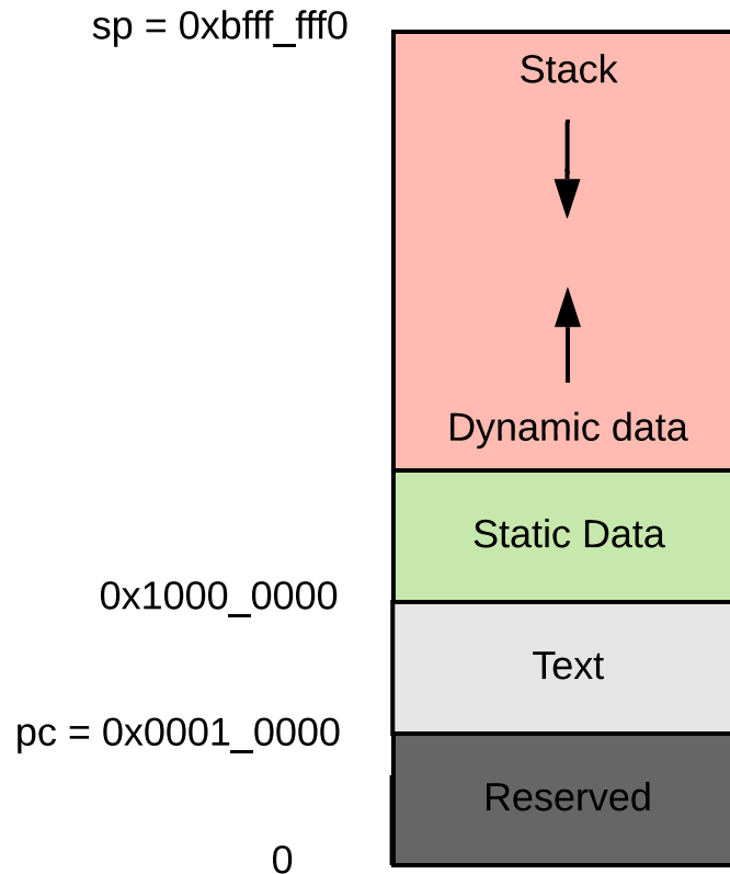
Figure 73: RV32 Memory Layout
