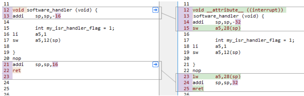
Figure 78: CLINT Interrupt Attribute Example
