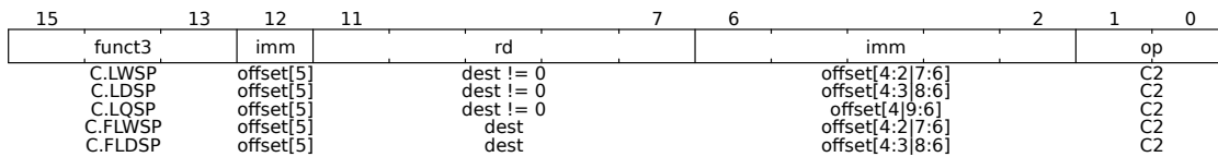
Figure 49: Stack-Pointed-Based Loads
