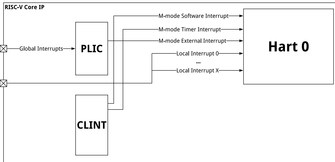
Figure 74: E34 Core Complex Interrupt Architecture Block Diagram
