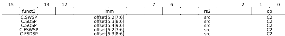
Figure 50: Stack-Pointed-Based Stores
