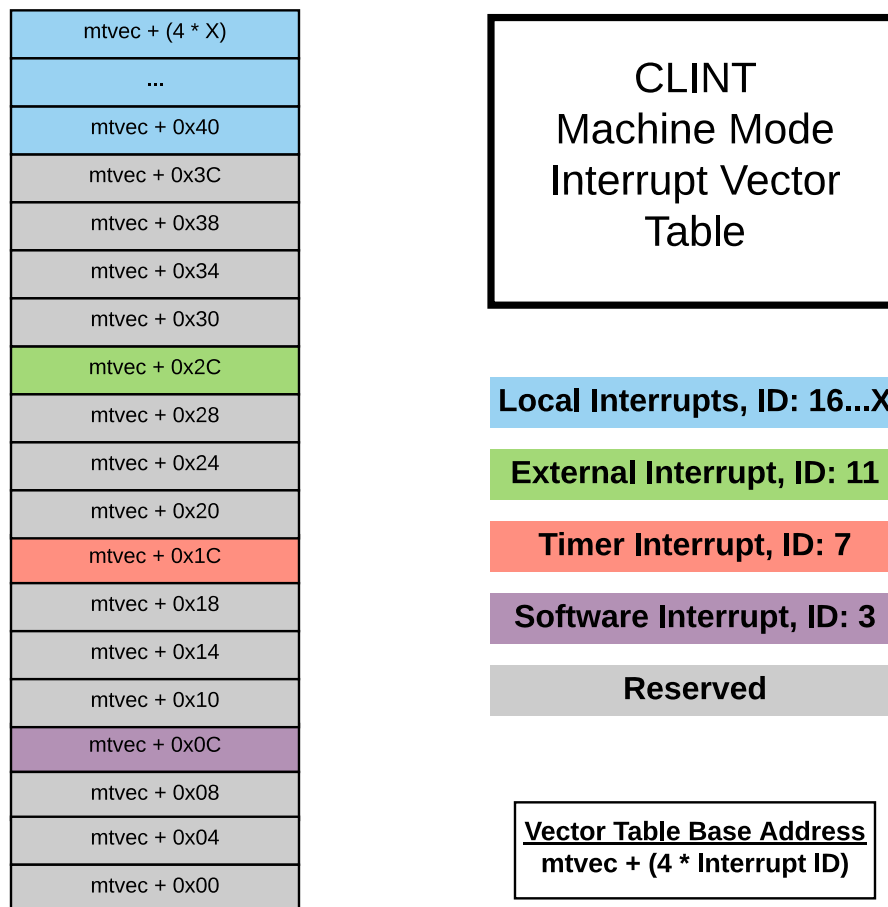
Figure 63: CLINT Interrupts and Vector Table
