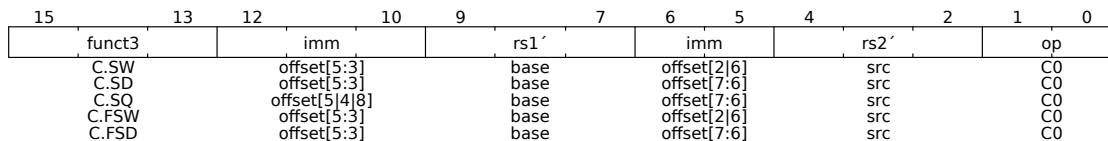
Figure 40: Register-Based Stores
