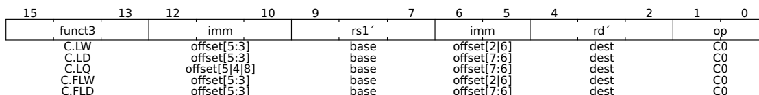
Figure 39: Register-Based Loads
