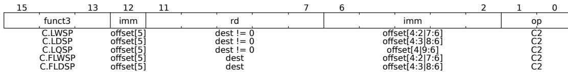
Figure 37: Stack-Pointed-Based Loads
