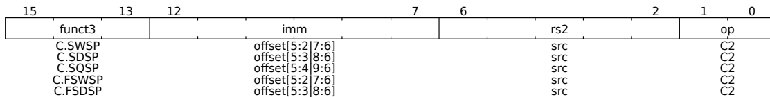
Figure 38: Stack-Pointed-Based Stores
