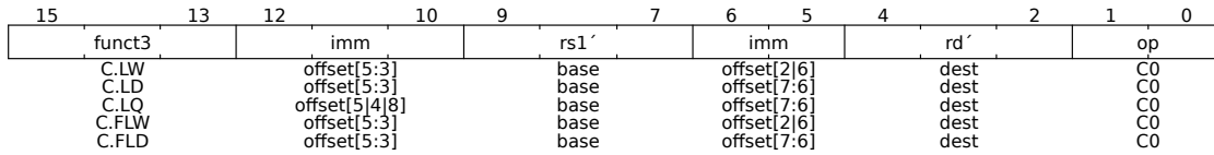
Figure 61: Register-Based Loads
