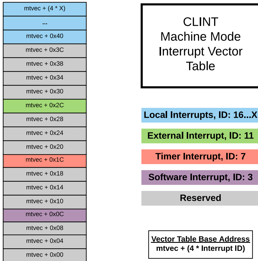
Figure 85: CLINT Interrupts and Vector Table
