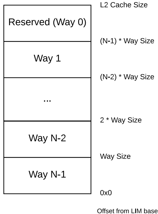
Figure 90: Mapping of L2 Cache Ways to L2 LIM Addresses
