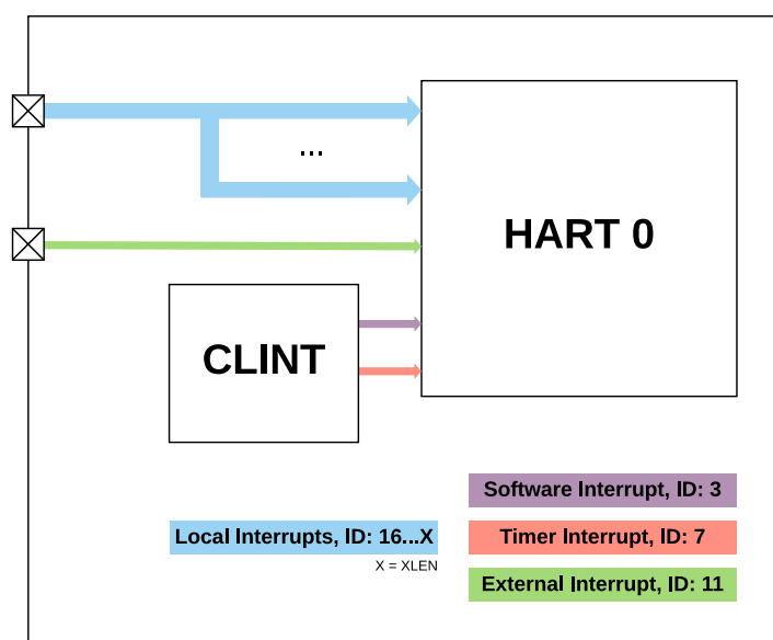
Figure 84: CLINT Block Diagram
