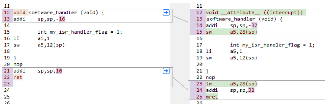
Figure 87: CLINT Interrupt Attribute Example
