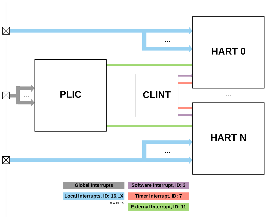
Figure 88: PLIC Multi-Core Block Diagram
