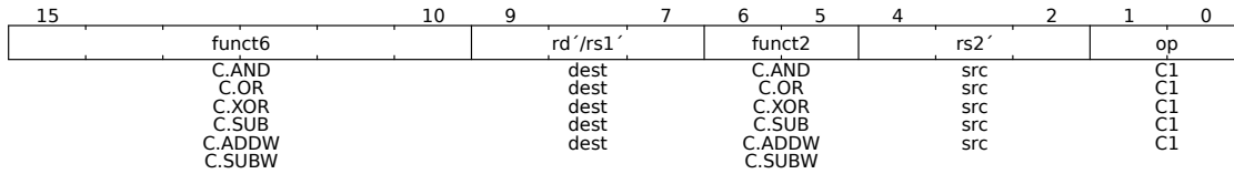
Figure 73: Integer Register-Register Operations (con't)
