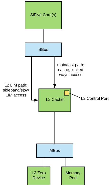
Figure 91: Difference between L2 LIM and L2 Zero Device
