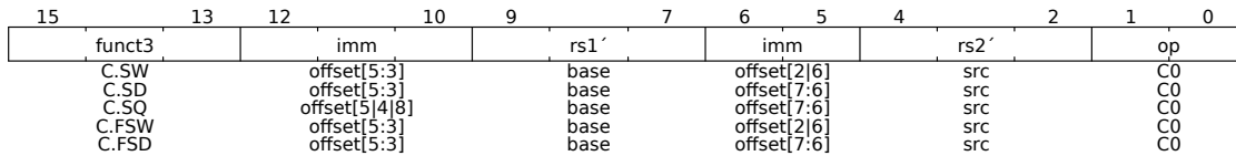
Figure 62: Register-Based Stores
