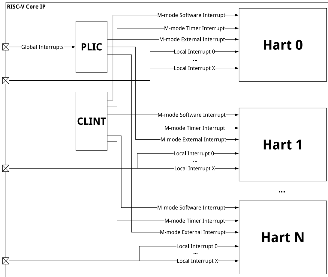
Figure 83: S76-MC Core Complex Interrupt Architecture Block Diagram
